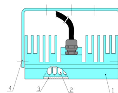
Picture 1. The IR-98 illuminator. Main view. 1 – case, 2 – luminodiodes, 3 – light filter, 4 – bracket
